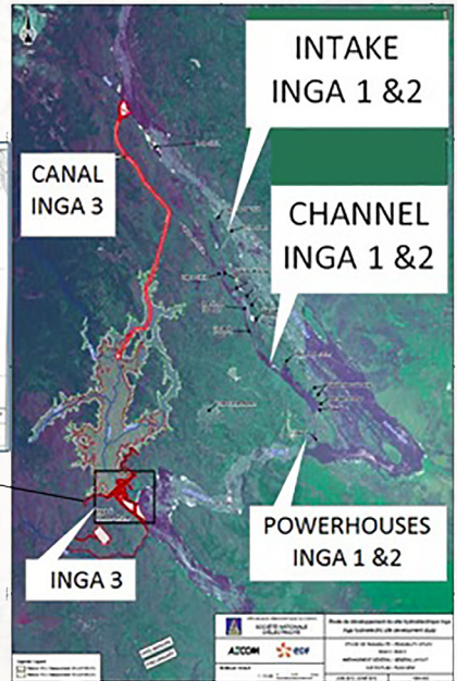
The proposed Inga 3 project, which includes a dam and a 4,800 MW hydroelectric plant at Inga Falls on the Congo River. Source: “The Inga 3 Hydropower Project,” International Rivers, http://www.internationalrivers.org/campaigns/the-inga-3-hydropower-project . Licensed under Creative Commons.
